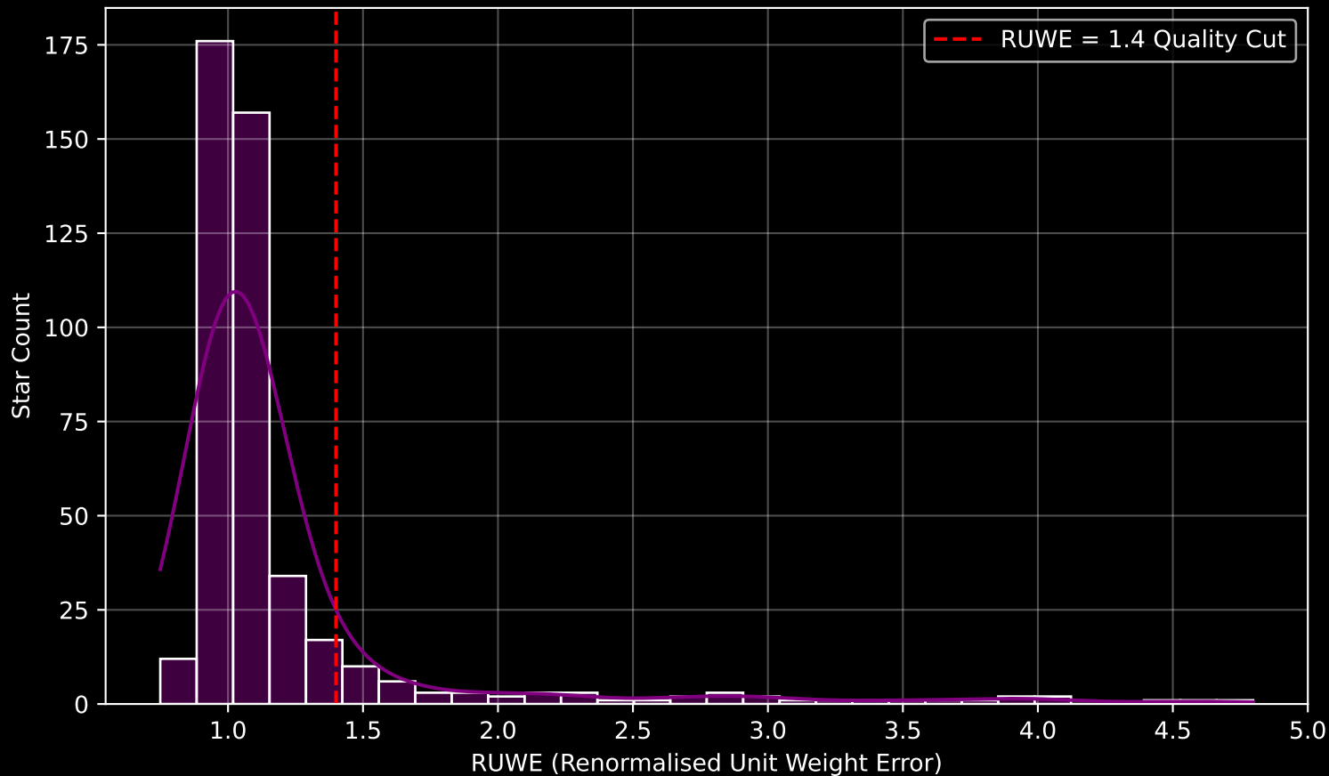
GALAH DR4 Field [6781] RUWE Distribution (n= 448)
