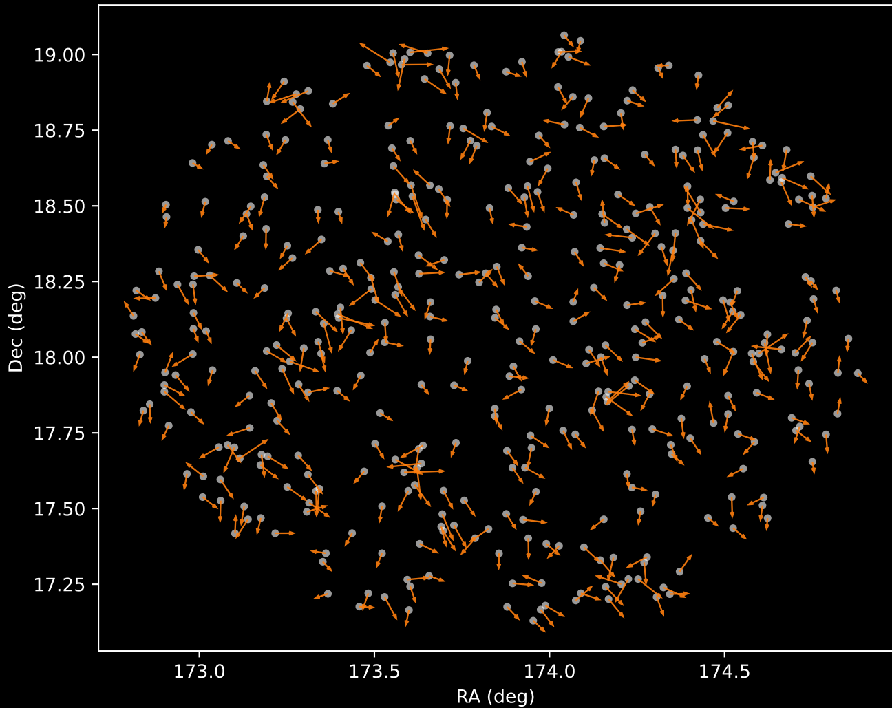
GALAH DR4 Cluster 2 Proper Motion Vectors (n=409)
