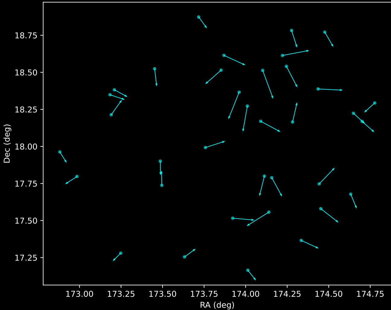
GALAH DR4 Noise Stream Proper Motion Vectors (n=36)
