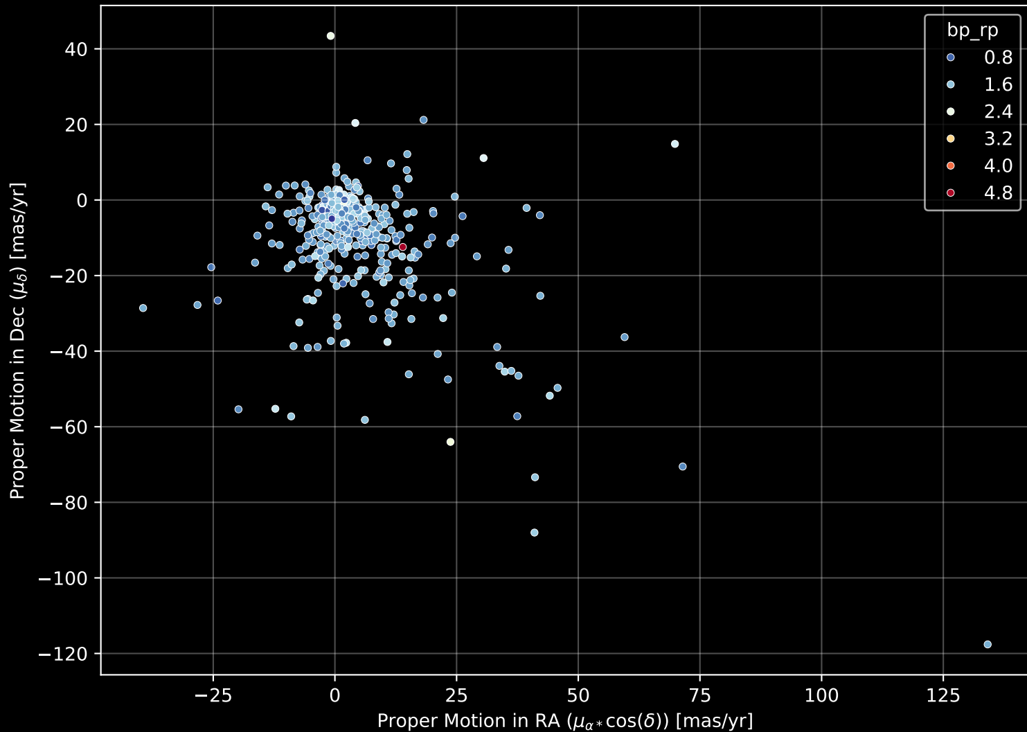
GALAH DR4 Field: [6781] Proper Motion Diagram (n= 459)
