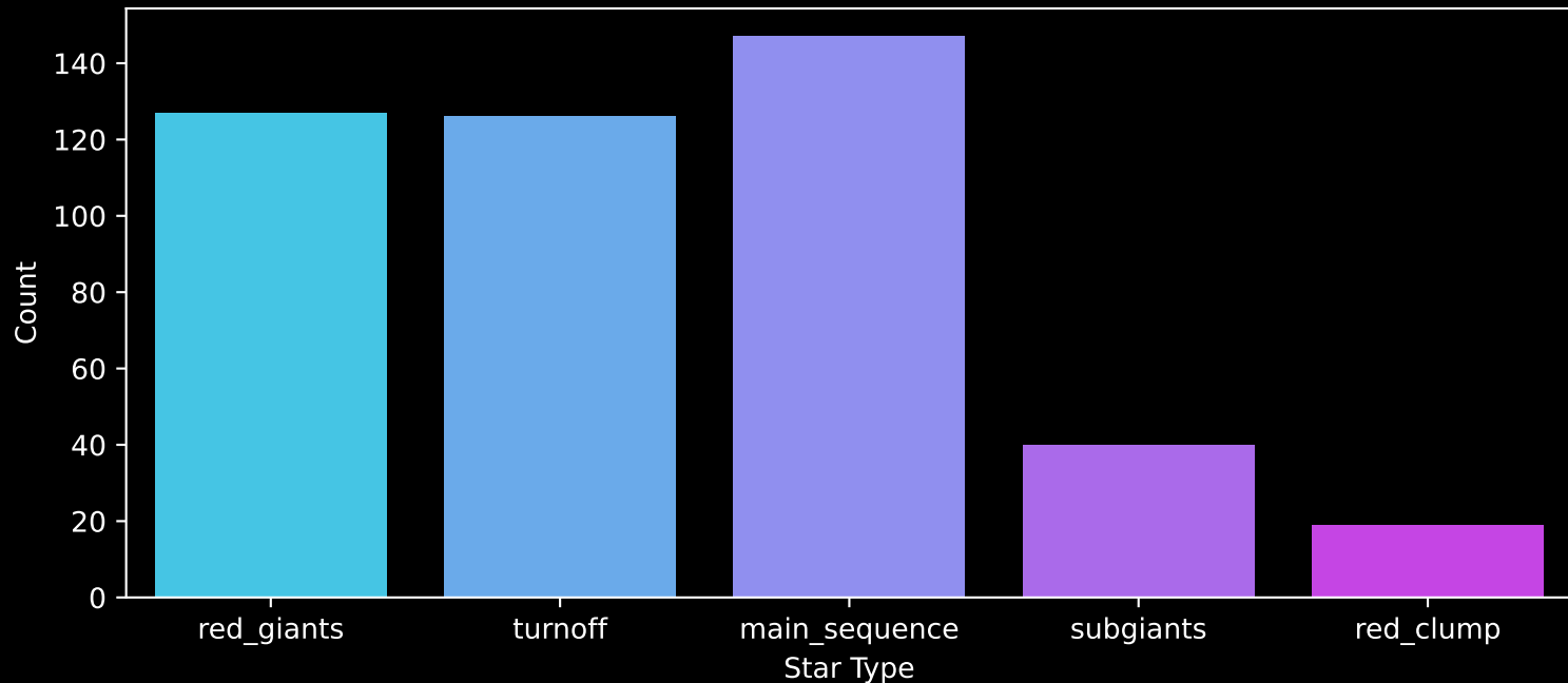
GALAH DR4 Field: [6781] Count plot of Star Type
